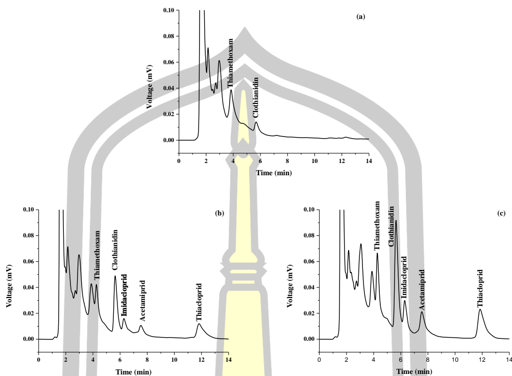
Figure 16. Chromatograms of (a) grape sample (super market), (b) grape sample spiked with 250 ng mL -1 of each neonicotinoid, and (c) grape sample spiked with 500 ng mL -1 of each neonicotinoid.
