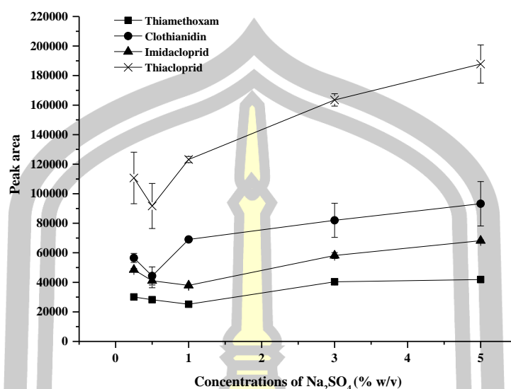
Figure 9. Effect of the amounts of salt. Conditions: 5 % (w/v) of \text{Na}_2\text{SO}_4 ; 25 % (w/v) of each surfactant; vortex time 30 sec; ultrasonication (I) temperature at 30 °C for 3 min; 100 \mu\text{L} of 1.00 mol \text{L}^{-1} \text{CHCl}_3 ; 100 \mu\text{L} of 1.00 mol \text{L}^{-1} phenol; ultrasonication (II) temperature at 60 °C for 20 min; centrifugation (I) time at 3000 rpm for 5 min; centrifugation (II) time at 3000 rpm for 1 min (sample volume 10 mL, 0.1 \mu\text{g mL}^{-1} of each neonicotinoid insecticide).
