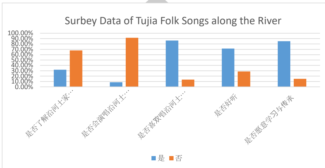
Figure 22 Questionnaire
