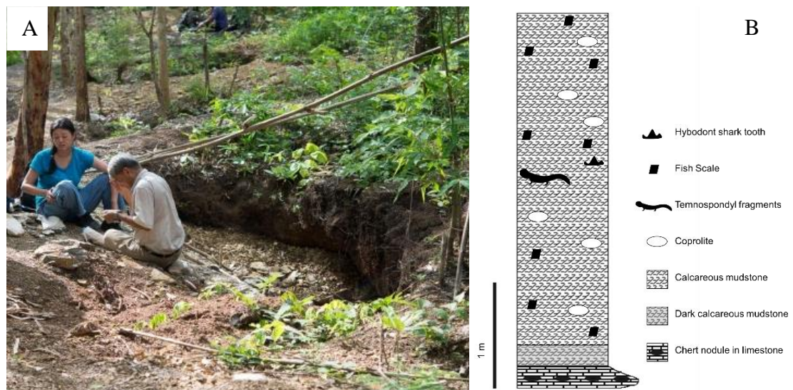
Figure 6 The Huai Nam Aun locality near the Nongyakong village, Khonsan district, Chaiphum province (A). The section of the Huai Nam Aun locality (B, modified from Laojumpon et al., 2012).
