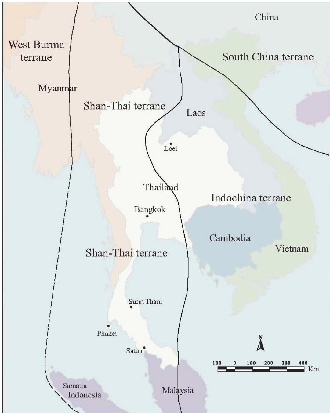
Figure 1 Map shows the boundary of tectonic terranes in Thailand (Department of Mineral Resources, 2014)
